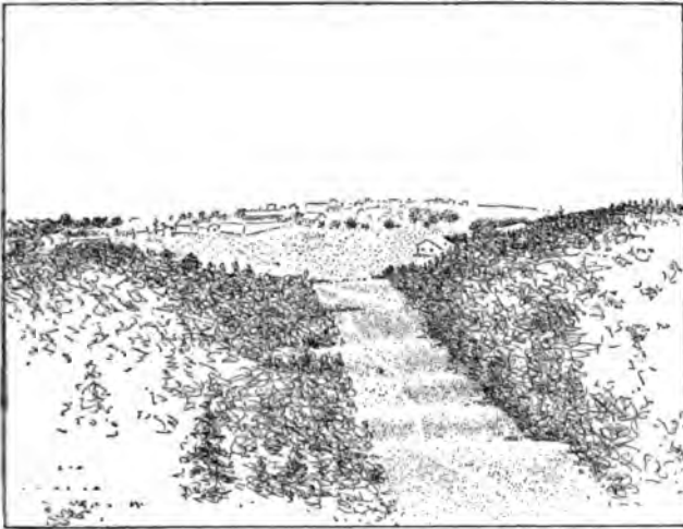
g. 371. — View from the observatory upon Mackinac Island across the "Short Target Range" toward the Fort. Beach ridges appear in succession within the cleared space (after a photograph by Rossiter).
